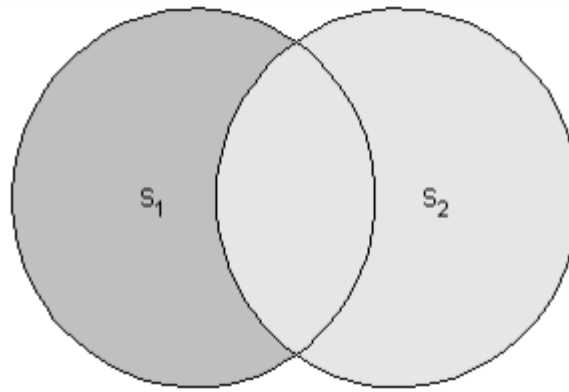
s_1.diff(s_2)
