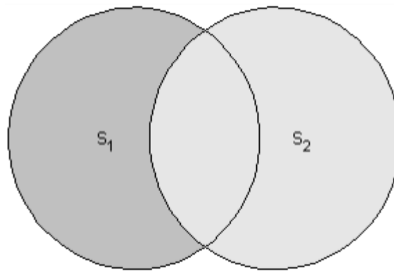
s_1.diff(s_2)
