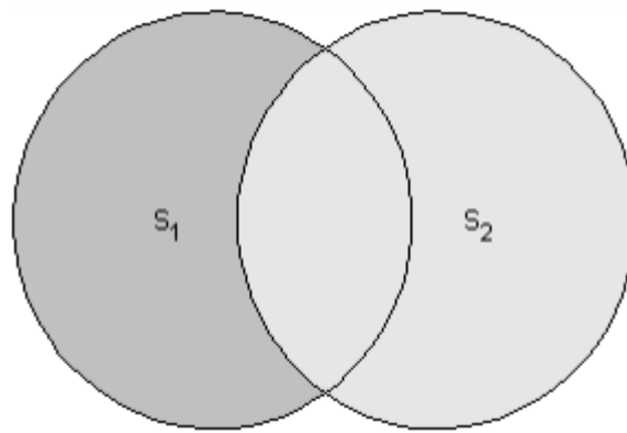
s_1.diff(s_2)
